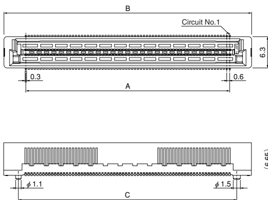
Top entry type
