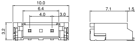
(2 circuits 4.0mm pitch)
