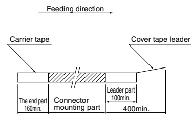
Top entry type <Staggered, Normal type> (9 circuits)
