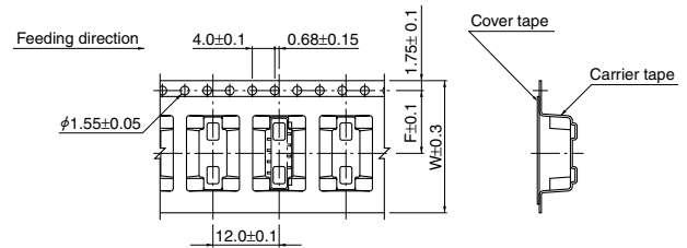
Top entry type <Staggered, Normal type> (9 circuits)
