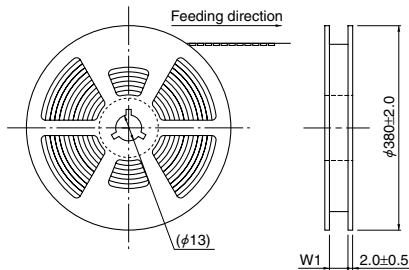
Top entry type <In-line, Normal type>
