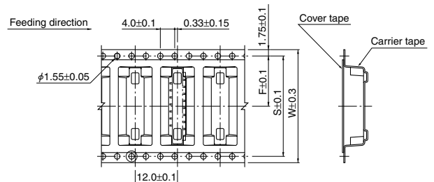
<Staggered, Large slider type> (22 circuits)
