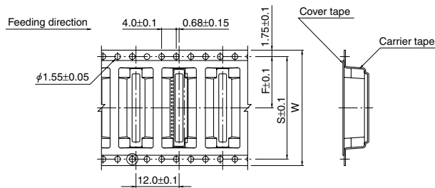
Top entry type <In-line, Reverse type>
