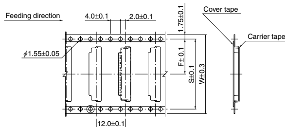
Side entry type <Normal type/Reverse type>
